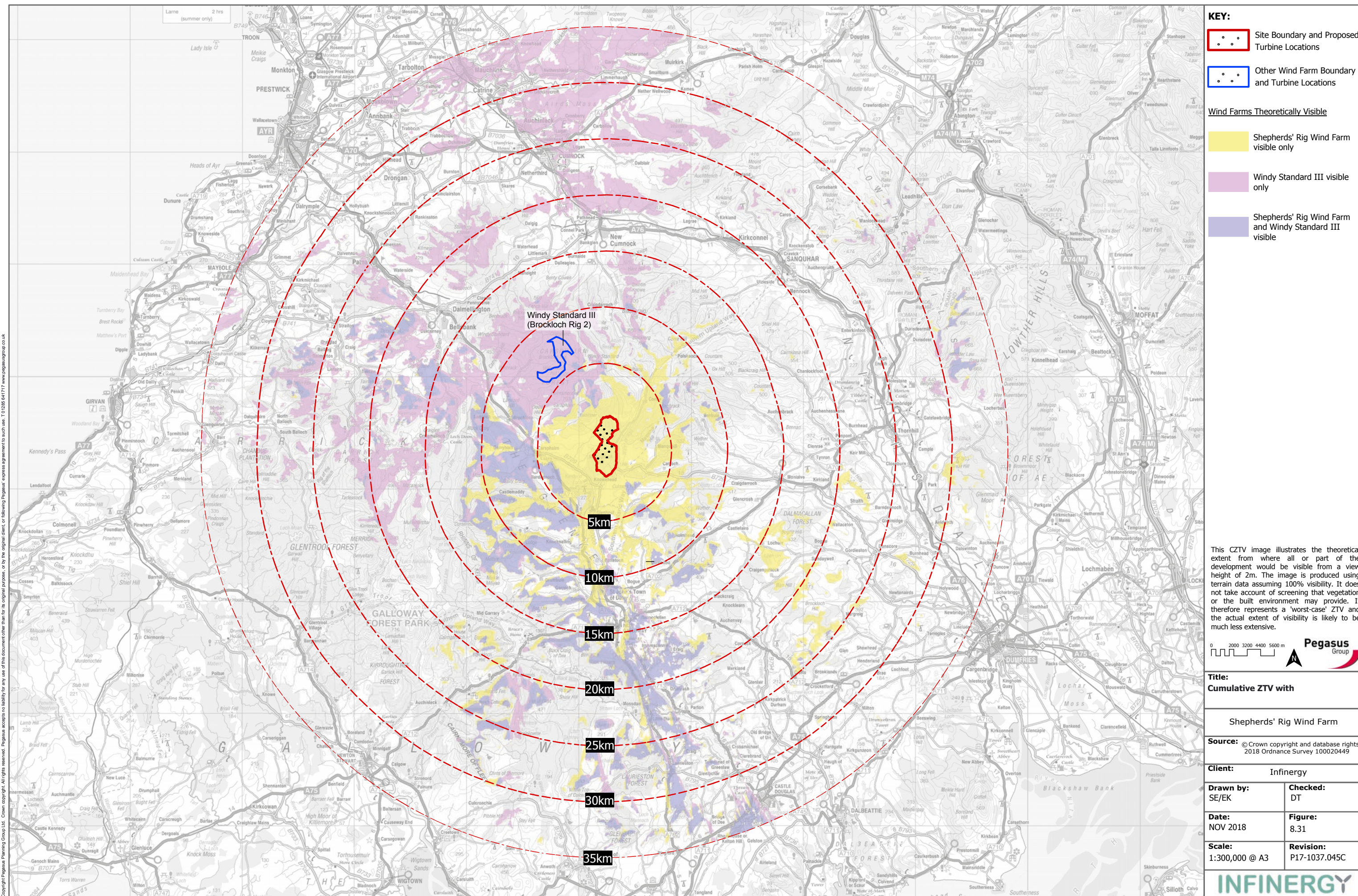
Figure 8.31 Cumulative ZTV with Windy Standard III
